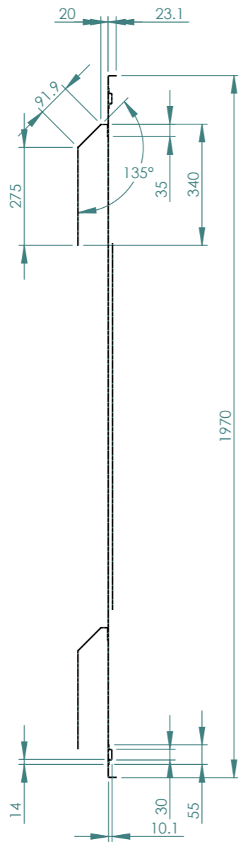
SECTION Q-Q
