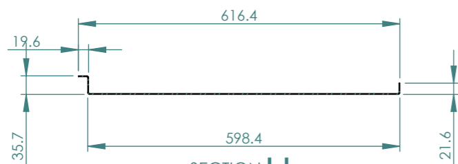
SECTION I-I
