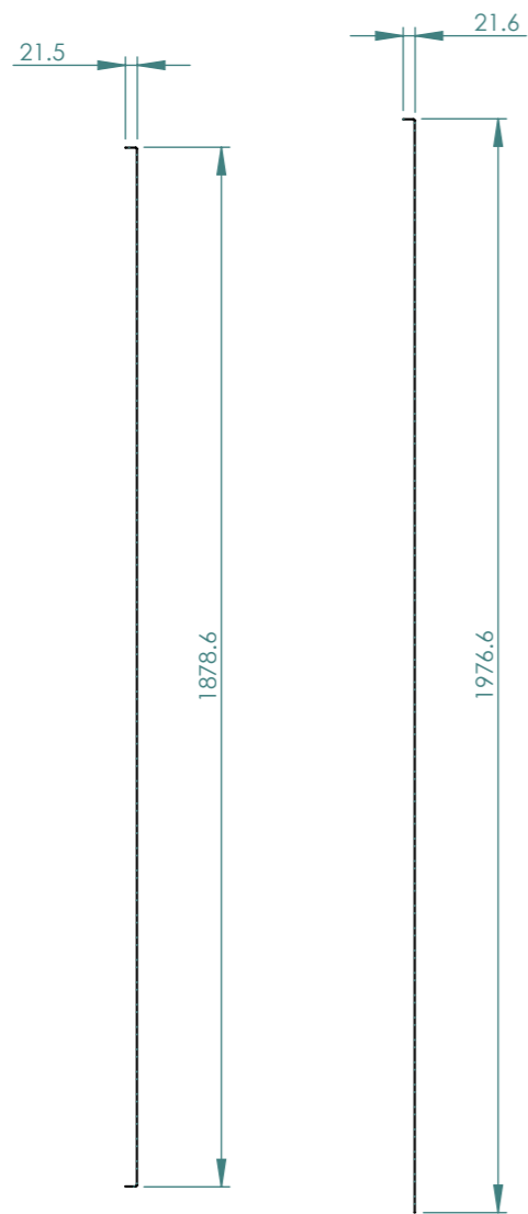
SECTION O-O
