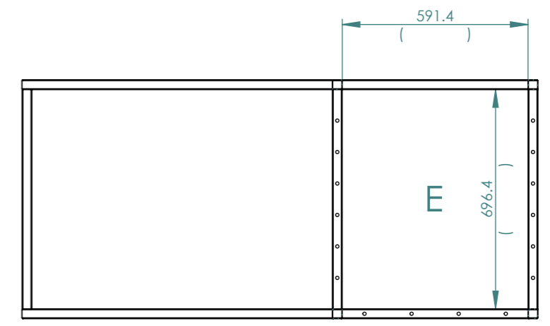
SECTION E-E
